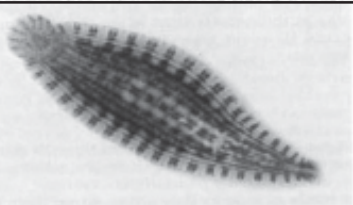
Gambar 9.14 Lintah (Sumber: http://alpha.fmarion.edu )
