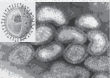
Gambar 3.8 Virus Influenza (Sumber: www.coloradoallergy.com dan www.voquelgrippe.bbraun.de )
